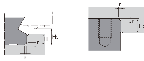
LM rail section
